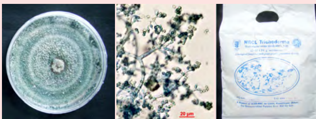
Culture of Trichoderma viride strain NRCL T-01 and trial pack of talc-based Trichoderma formulation
